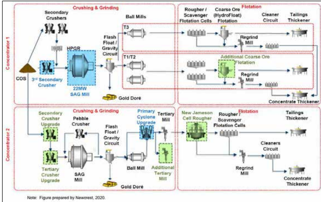
Figure 2.14 Simplified process flow sheet for Concentrator 1 & 2
